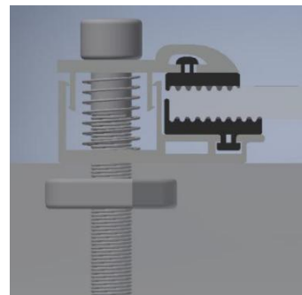
One-side briquetting illustration
